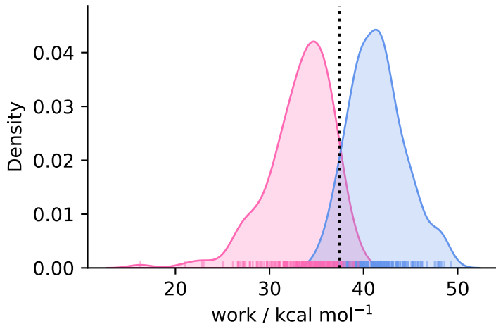
complex ( N = 199 )
