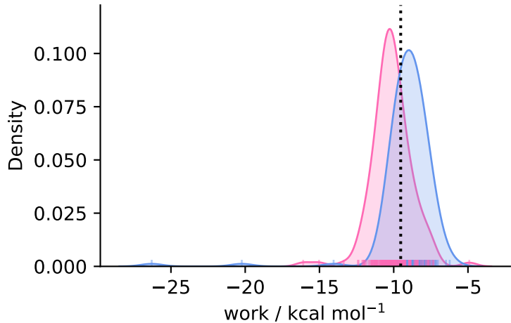
complex ( N = 145 )
