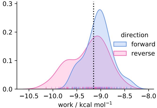
solvent ( N = 84 )
