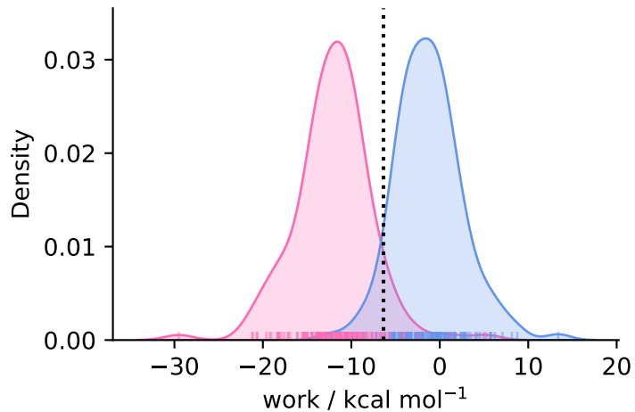
complex ( N = 138 )
