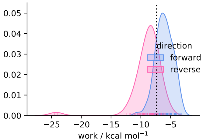
solvent ( N = 90 )
