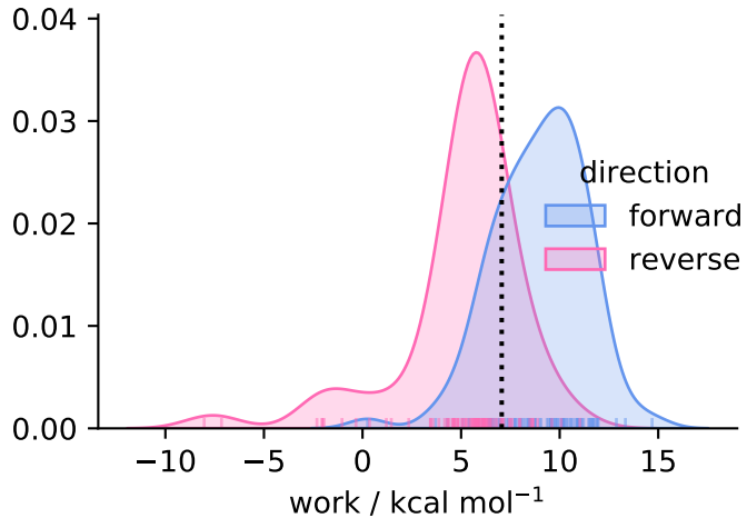
solvent ( N = 89 )
