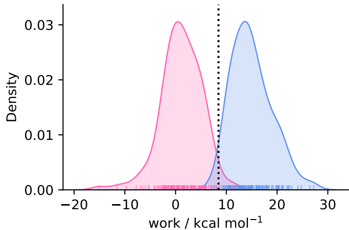
complex ( N = 140 )
