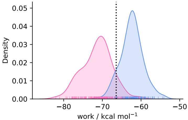
complex ( N = 150 )
