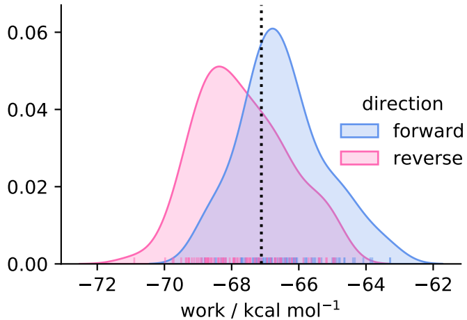
solvent ( N = 87 )
