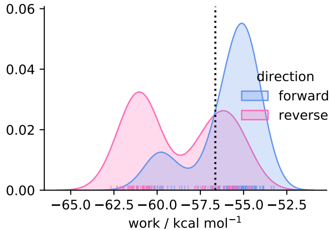
solvent ( N = 90 )
