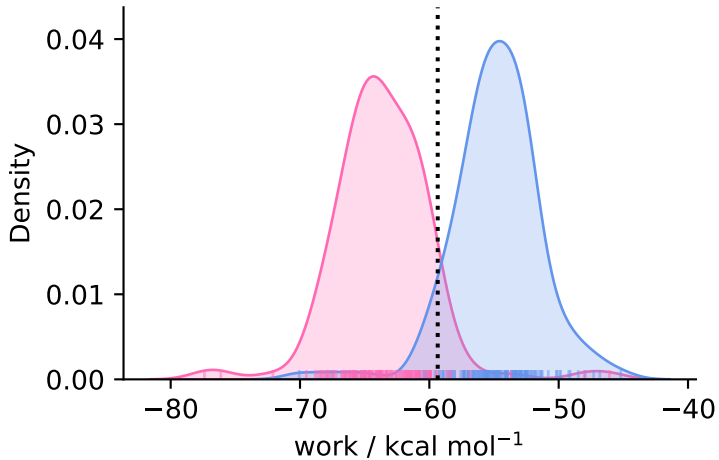
complex ( N = 140 )
