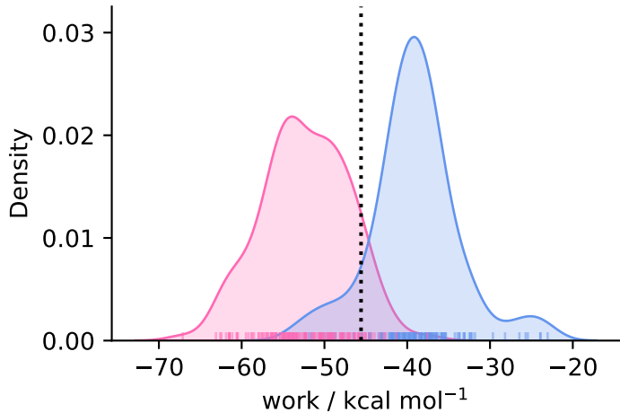
complex ( N = 143 )
