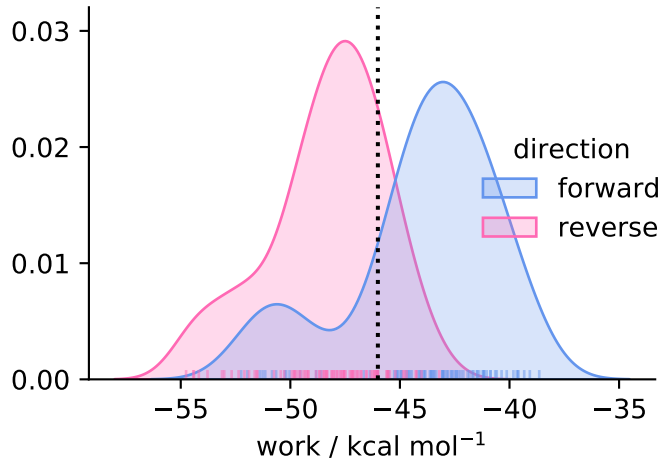
solvent ( N = 85 )
