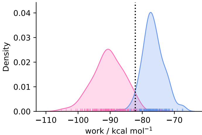
complex ( N = 150 )
