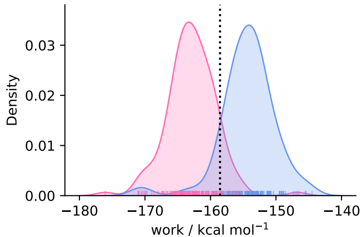
complex ( N = 135 )
