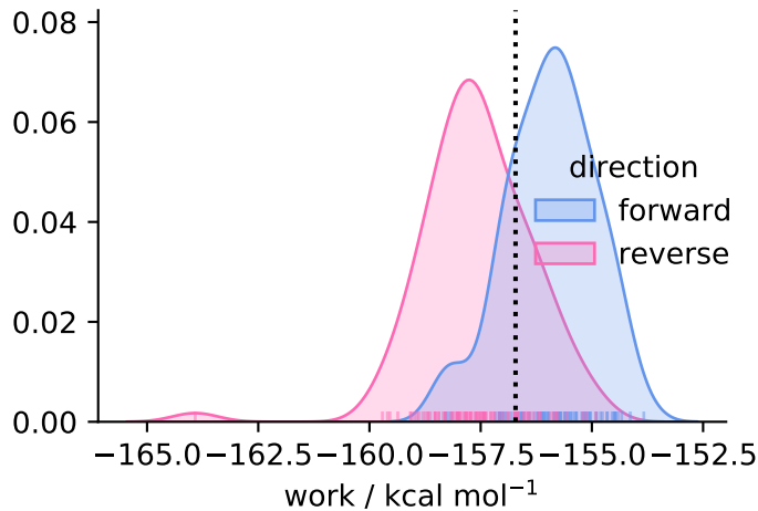
solvent ( N = 89 )
