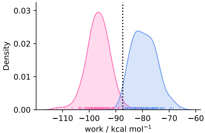
complex ( N = 141 )
