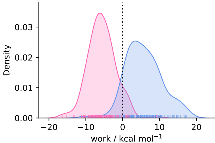
complex ( N = 136 )
