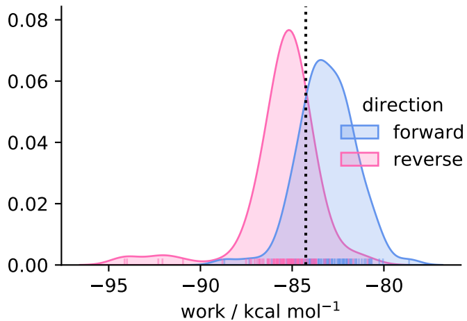
solvent ( N = 100 )
