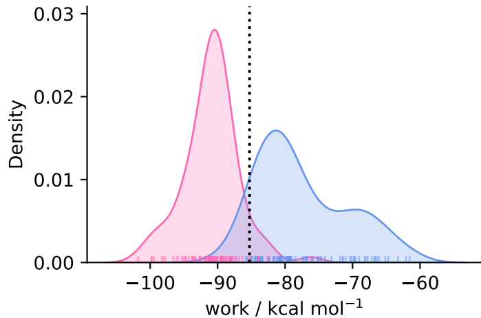
complex ( N = 89 )
