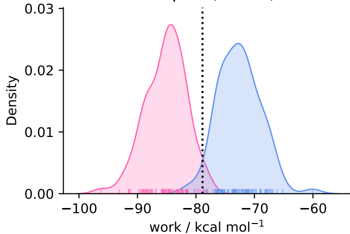
complex ( N = 90 )
