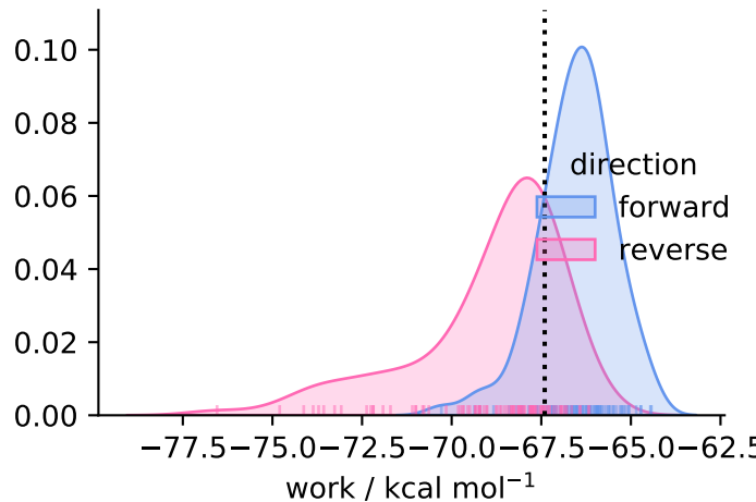
solvent ( N = 100 )
