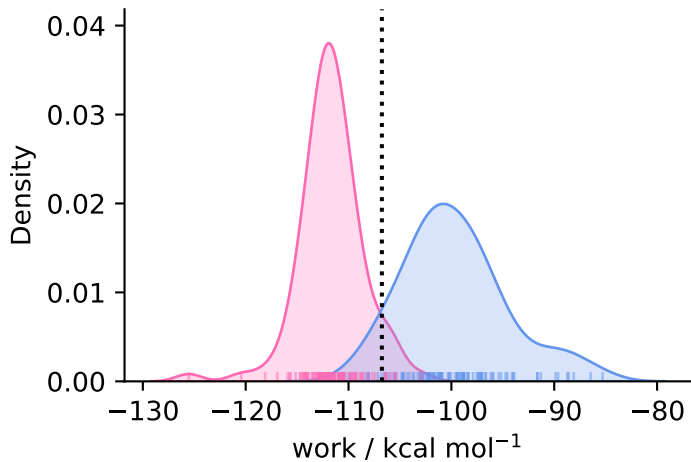
complex ( N = 96 )
