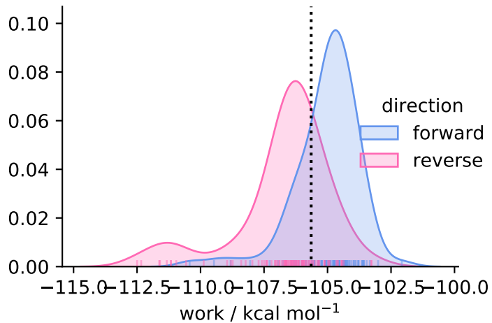
solvent ( N = 99 )
