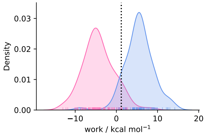
complex ( N = 93 )
