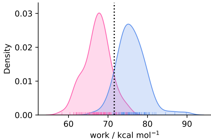
complex ( N = 92 )
