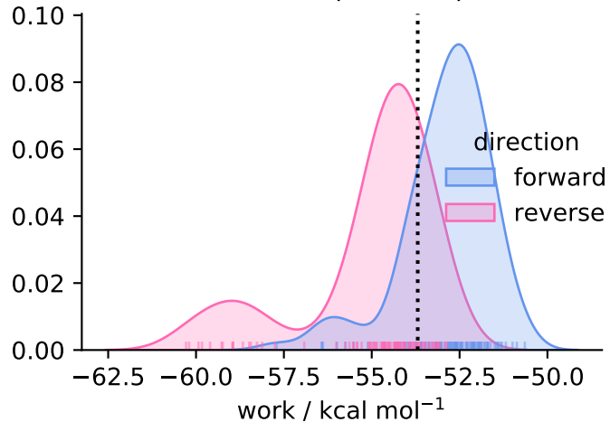
solvent ( N = 100 )
