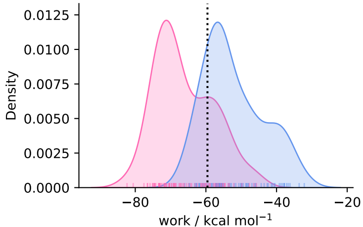
complex ( N = 87 )
