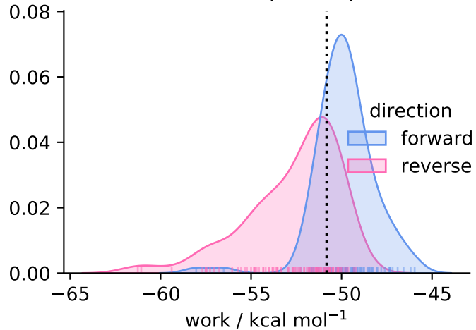
solvent ( N = 98 )
