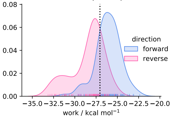
solvent ( N = 99 )
