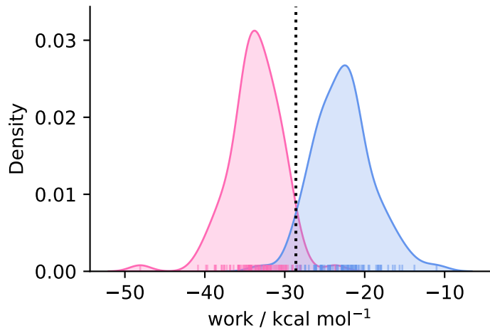
complex ( N = 91 )
