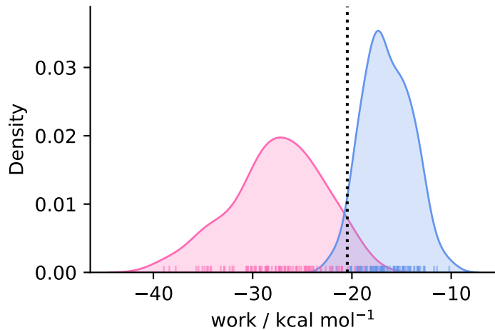
complex ( N = 90 )
