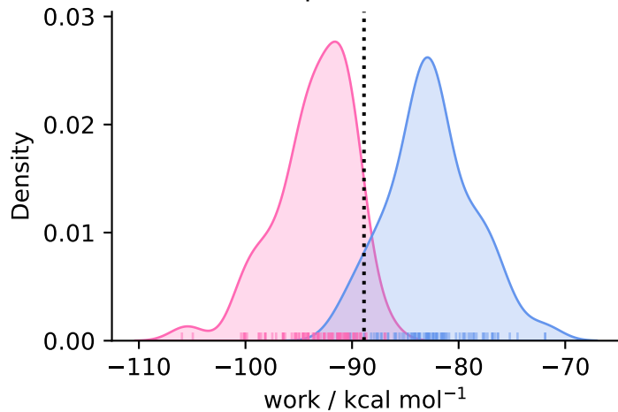
complex ( N = 95 )
