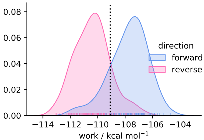
solvent ( N = 97 )
