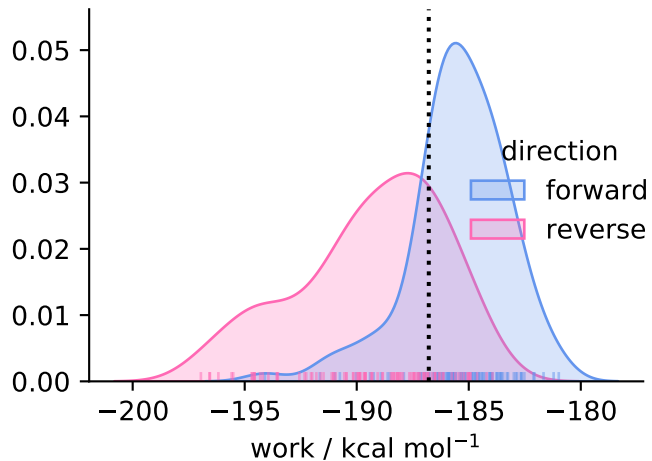
solvent ( N = 100 )
