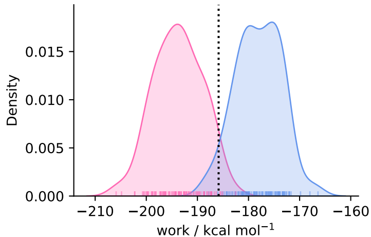
complex ( N = 93 )
