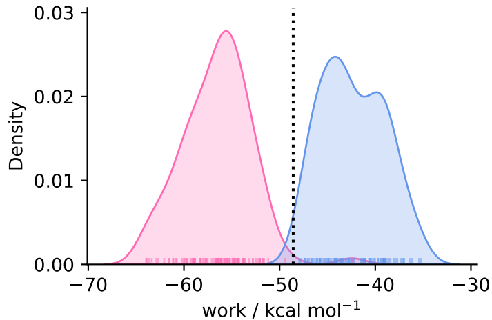
complex ( N = 94 )
