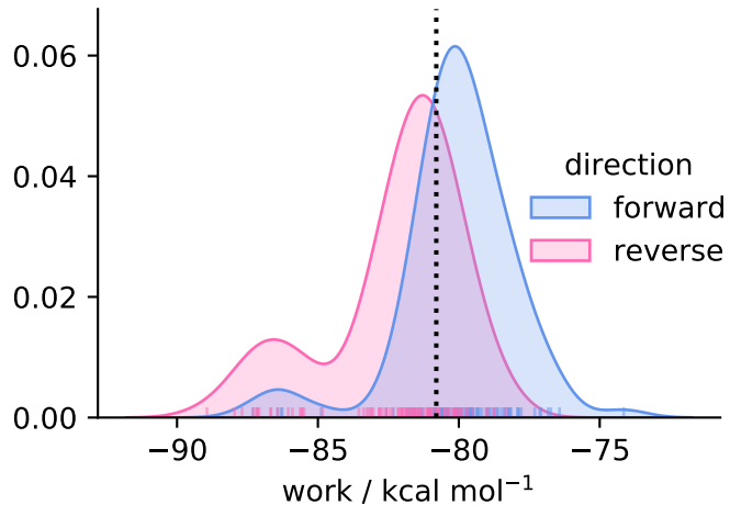
solvent ( N = 98 )
