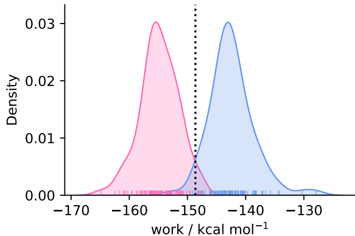
complex ( N = 96 )
