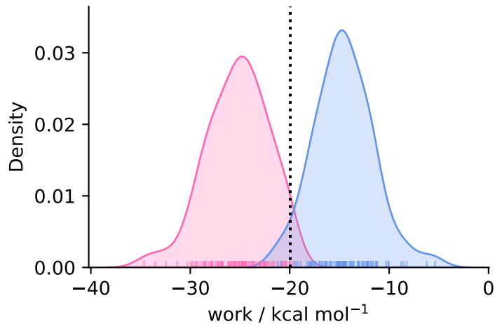
complex ( N = 97 )
