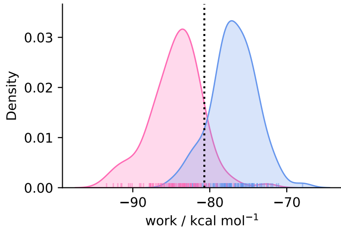
complex ( N = 99 )
