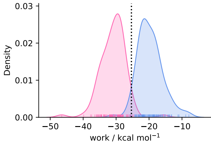
complex ( N = 97 )
