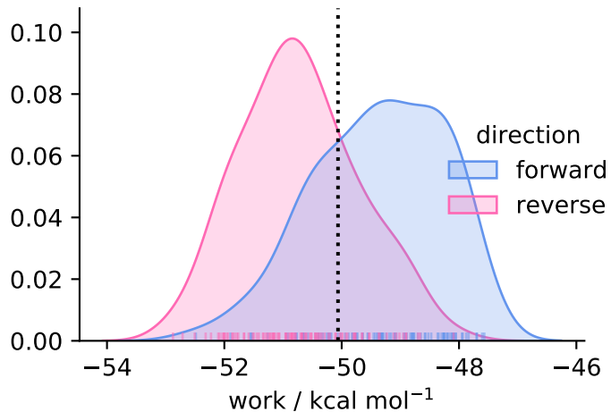
solvent ( N = 98 )
