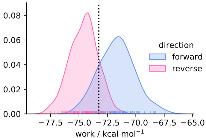
solvent ( N = 99 )
