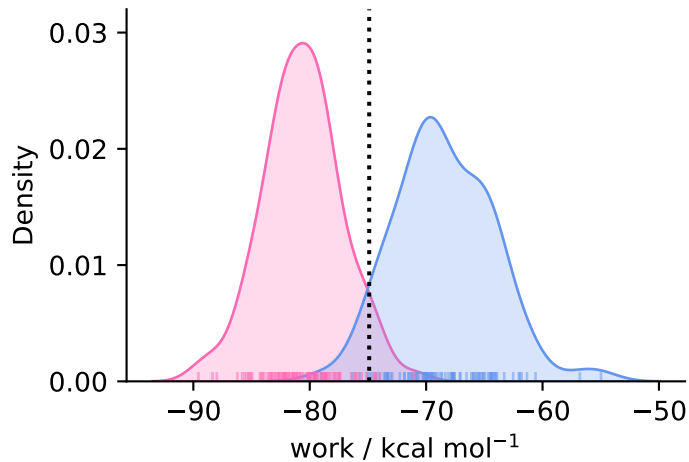
complex ( N = 97 )
