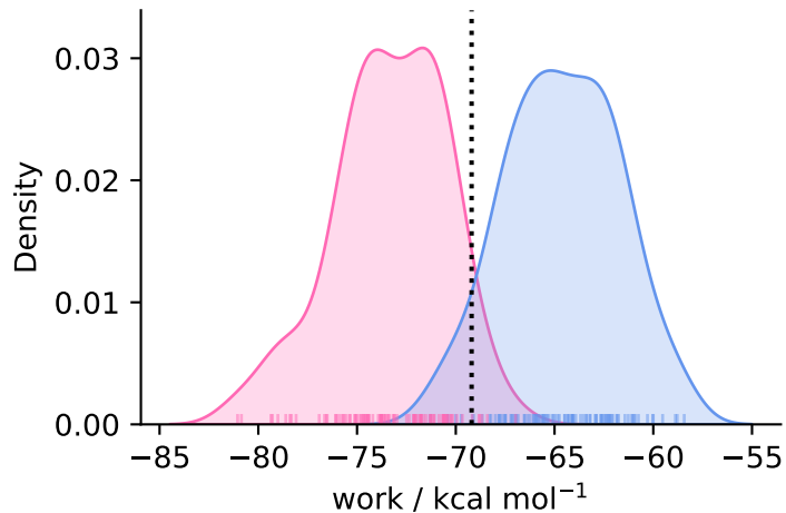
complex ( N = 98 )
