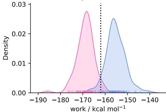
complex ( N = 96 )
