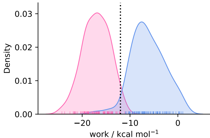
complex ( N = 98 )
