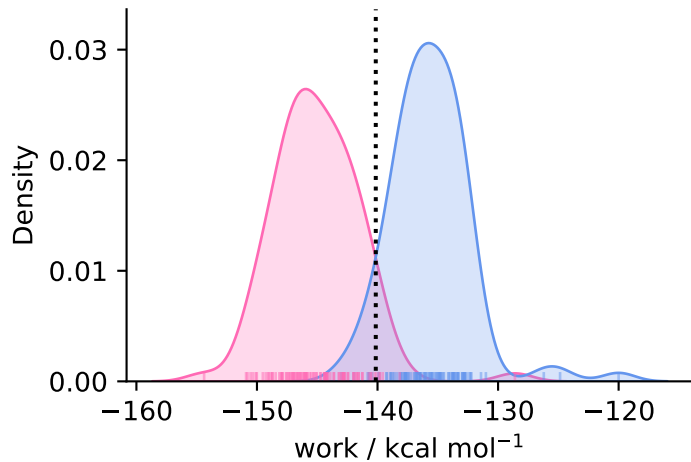
complex ( N = 94 )
