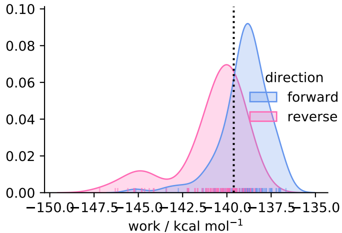
solvent ( N = 99 )
