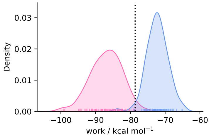
complex ( N = 92 )
