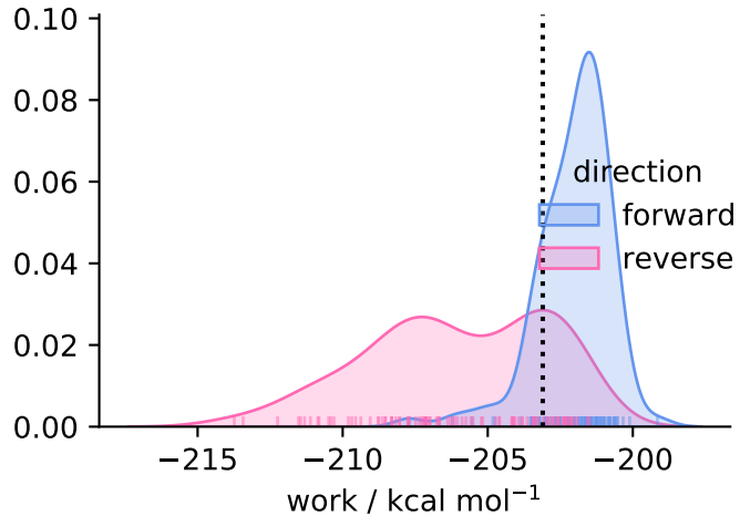
solvent ( N = 100 )
