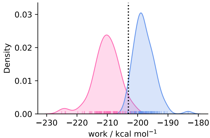
complex ( N = 99 )
