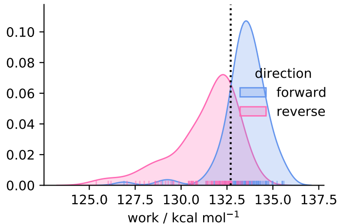
solvent ( N = 99 )
