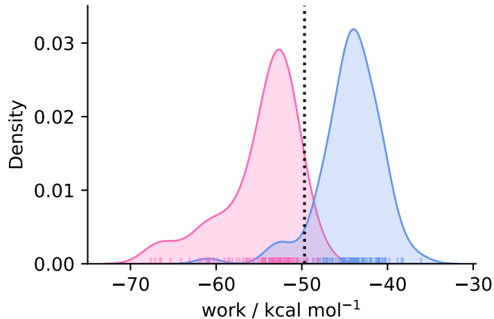
complex ( N = 96 )
