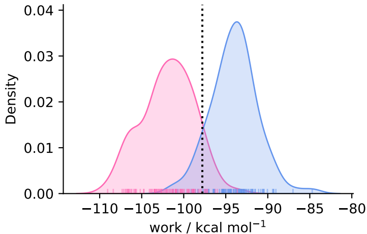
complex ( N = 97 )
