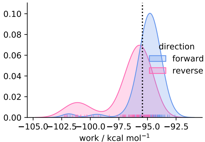
solvent ( N = 100 )
