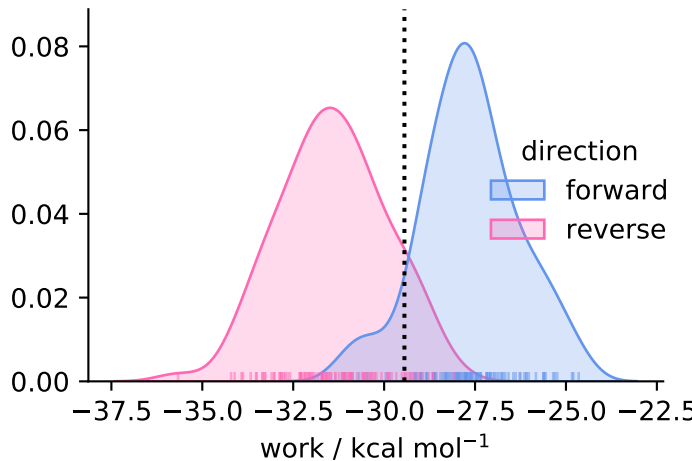
solvent ( N = 99 )
