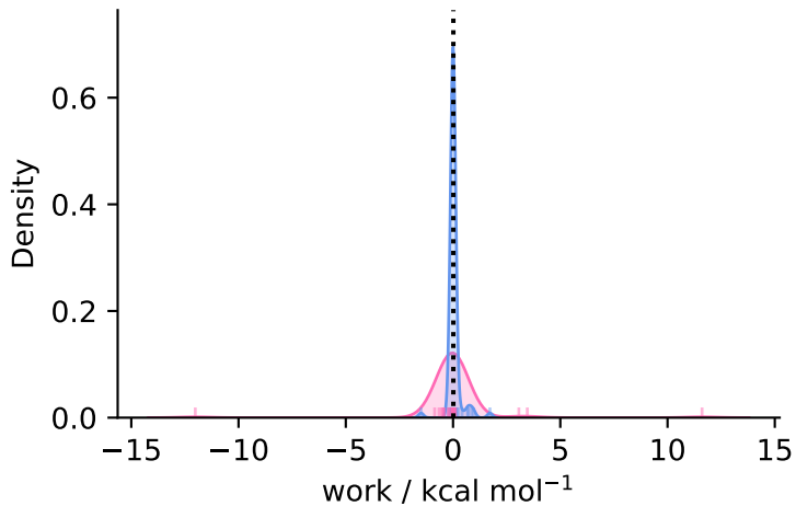
complex ( N = 92 )
