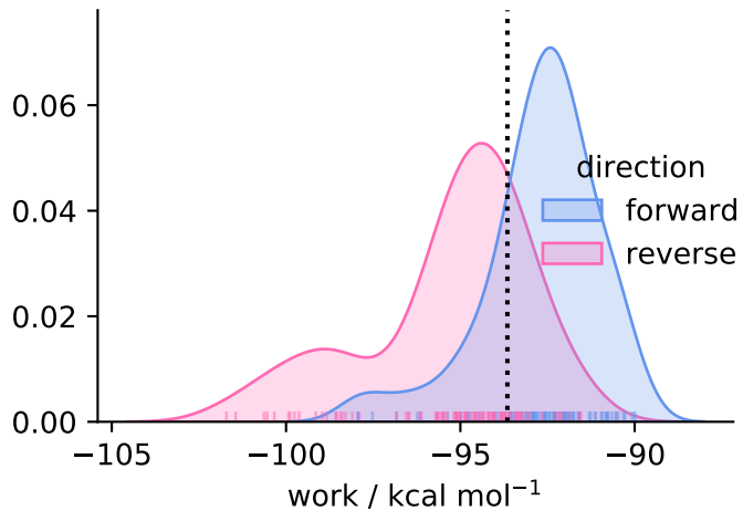
solvent ( N = 95 )
