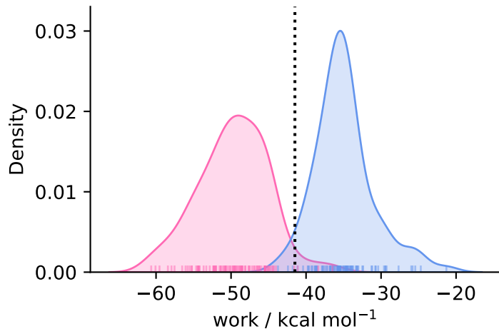
complex ( N = 90 )
