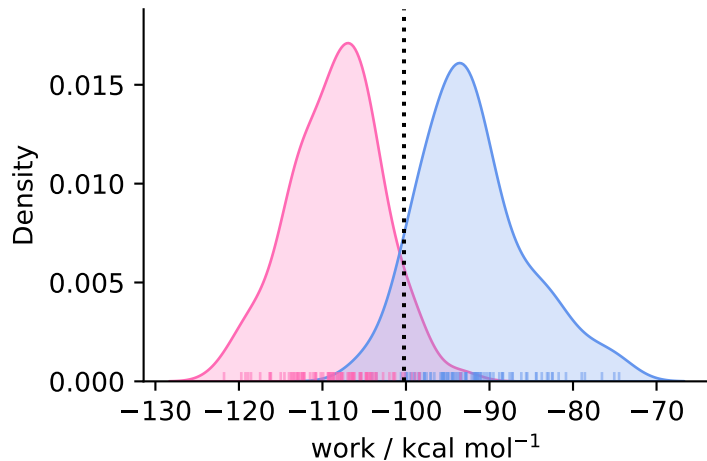
complex ( N = 91 )
