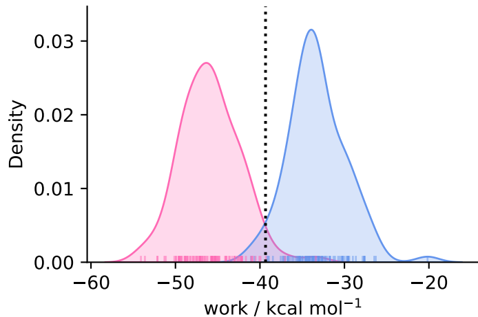
complex ( N = 95 )
