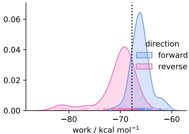
solvent ( N = 100 )
