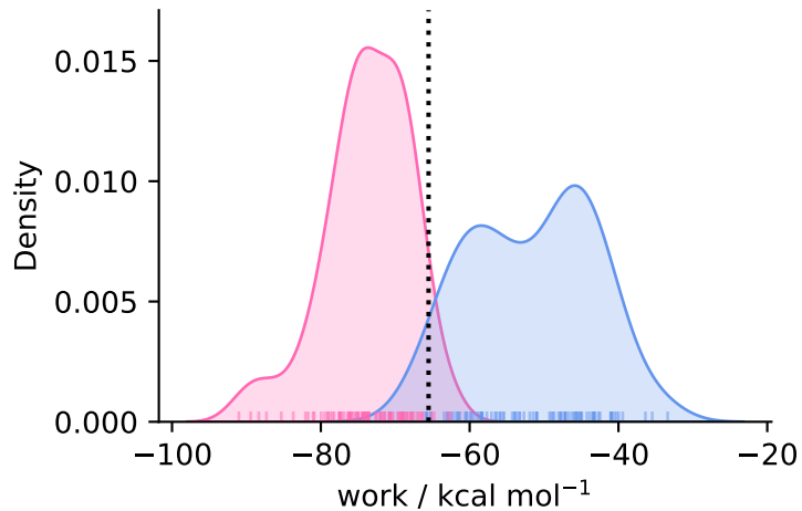
complex ( N = 90 )
