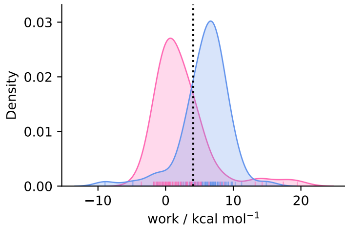
complex ( N = 71 )
