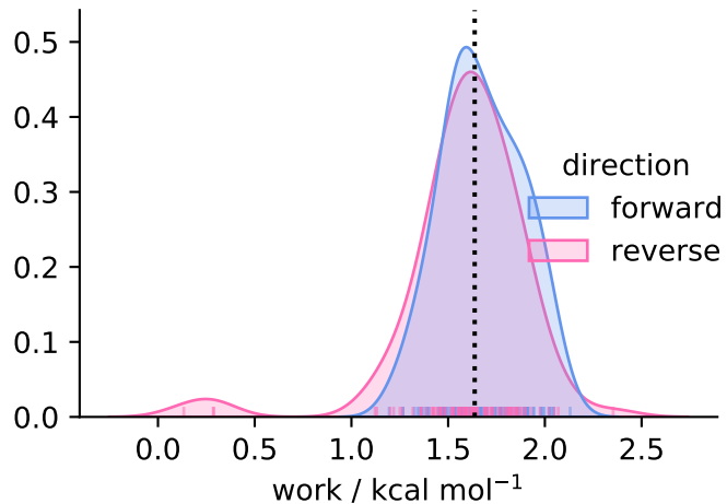
solvent ( N = 96 )
